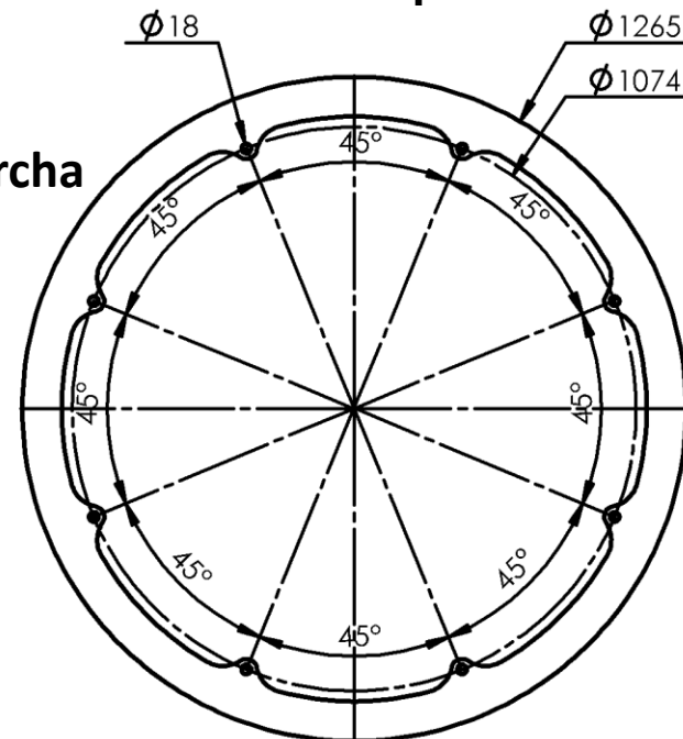
Anel superior
